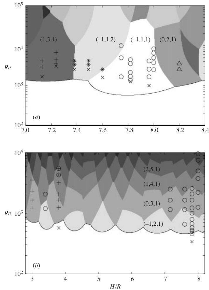
FIGURE 9. Comparison of the predicted and observed principal mode as a function of the experimental control parameters (H/R, Re) for (a) n = 2 and (b) n = 3 . Each grey tone corresponds to the most dangerous principal mode, i.e. the mode with the largest growth rate. The symbols represent experiments: (a) \circ , (-1, 1, 1) ; * , (-1, 1, 2) ; \triangle , (0, 2, 1) ; + , (1, 3, 1) and (b) \circ , (-1, 2, 1) ; + , (0, 3, 1) ; \times , visualizations where no distinct mode was observed.
